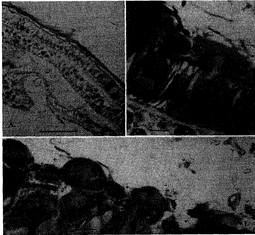
Fig. 1. (A) Light micrographic section of Montastrea annularis showing the coral epidermis, mesoglea, and gastrodermis, with coelenteron and calicoblast. The aragonitic skeleton has been removed, but normally would appear in the lower left portion of the field. Note the intact and continuous thin mucus layer over the epidermis in the right upper field. Marker = 0.1mm.; (B) Light micrographic section of M. annularis showing the appearance of the mucus layer in Rapid wasting disease. The mesoglea separates the epidermis from the zooxanthellate gastrodermis. Marker = 0.01mm.; (C) Another section of M. annularis with Rapid wasting disease, showing fungal hyphae ( ^ ) adjacent to the epidermis. Marker = 0.01mm. In both (B) and (C) the mucous layer, instead of being integrated into a continuous thin film over the coral epidermis, is eroded and unconsolidated, appearing as mucus pitting ( * ) and as individual globules. These abnormal features indicate the breakdown of the usually protective mucous barrier over the coral epithelium. Plastic embedded sections stained with Toluidine Blue 10B.
