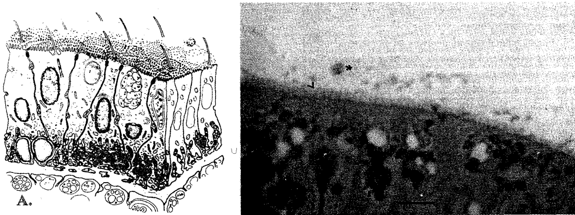
Fig. 2. (A) Diagram of coral planula of Porites porites showing microvilli and flagellae of the epidermis. Original diagram by R. Hayes (Hayes and Goreau, 1977); (B) Section of P. porites planular epidermis stained with potassium permanganate to show microvilli ( ^ ) and flagellae ( * ). Marker = 0.01mm.
