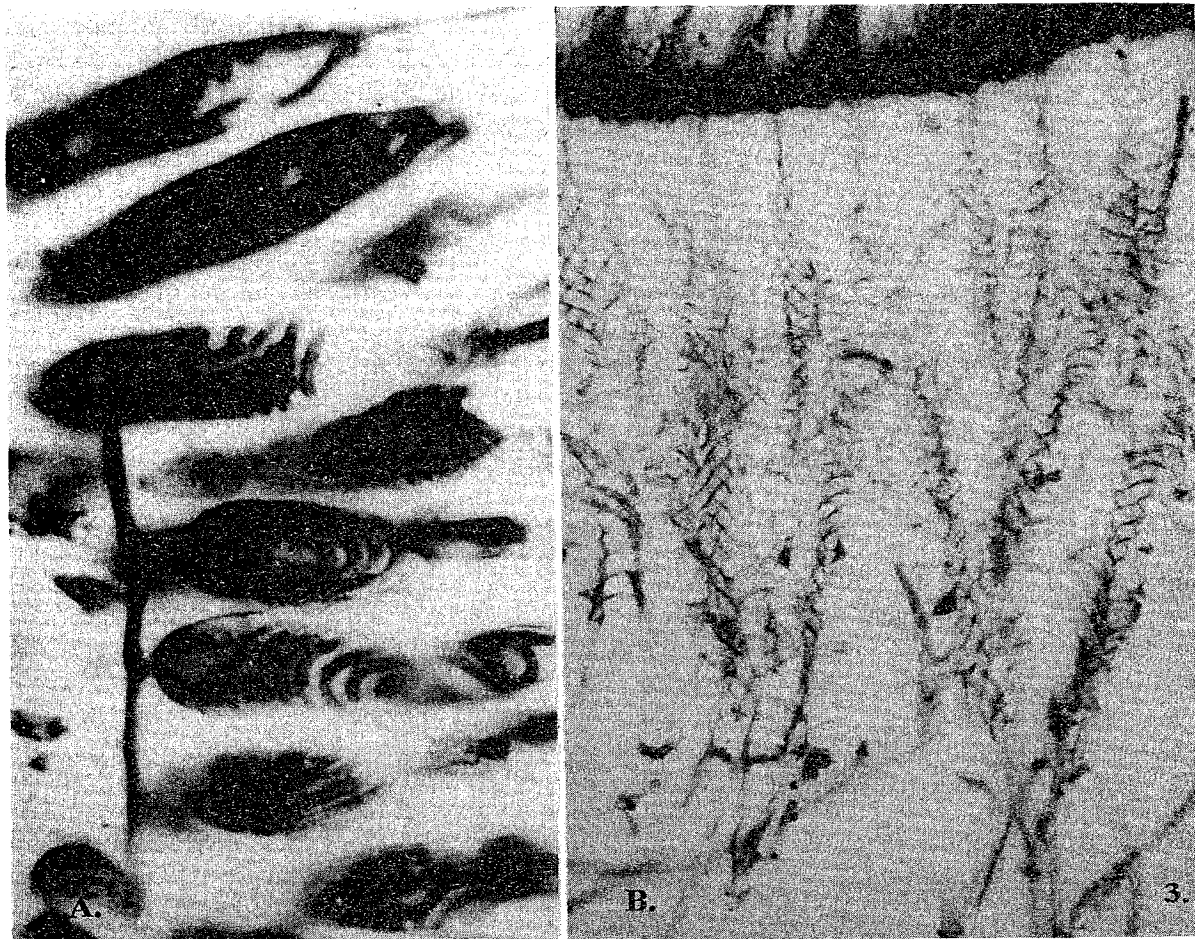
Fig. 3. Coral nematocysts in situ. (A) Light micrograph showing en face view of nematocysts in whole mount of coral tissues; (B) Barbed nematocysts released from vesicles in the coral epidermis. Photos by T.F. Goreau.
